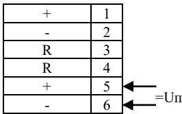
а) BC-07e-3(И)-24VDC
